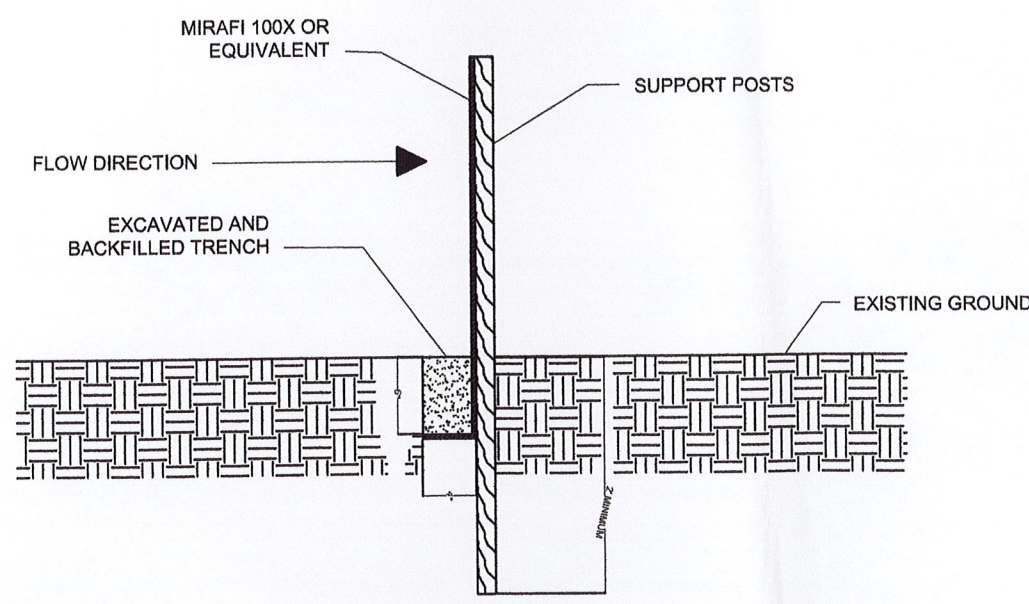
TYPICAL SECTION
